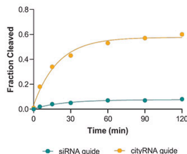
Figure 15. cityRNA enhances AGO2-RISC catalytic turnover, producing more rapid and greater cumulative product formation than siRNA.
