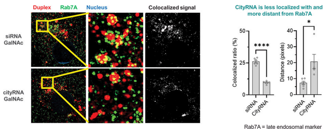
Figure 13. Reduced co-localization of cityRNA-GalNAc with the late endosomal marker Rab7A compared to siRNA-GalNAc.
