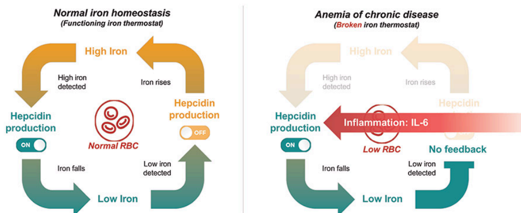
Figure 8: Anemia of chronic disease short-circuits the body's iron thermostat: iron homeostasis requires feedback between liver and bloodstream through hepcidin.
